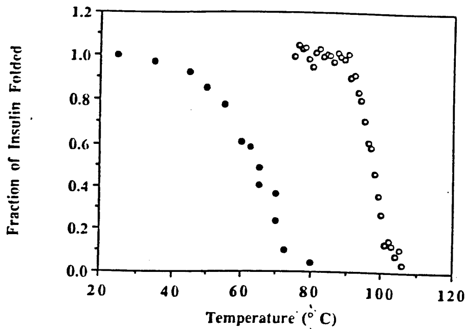
FIG. 6. The effect of temperature on the denaturation of insulin dissolved in water (●) and 1-octanol (○). The fraction folded was determined by monitoring the molar ellipticity at 222 nm.
